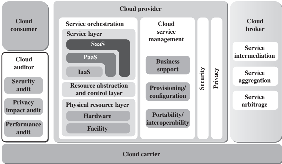
Figure 5.14 NIST Cloud Computing Reference Architecture
