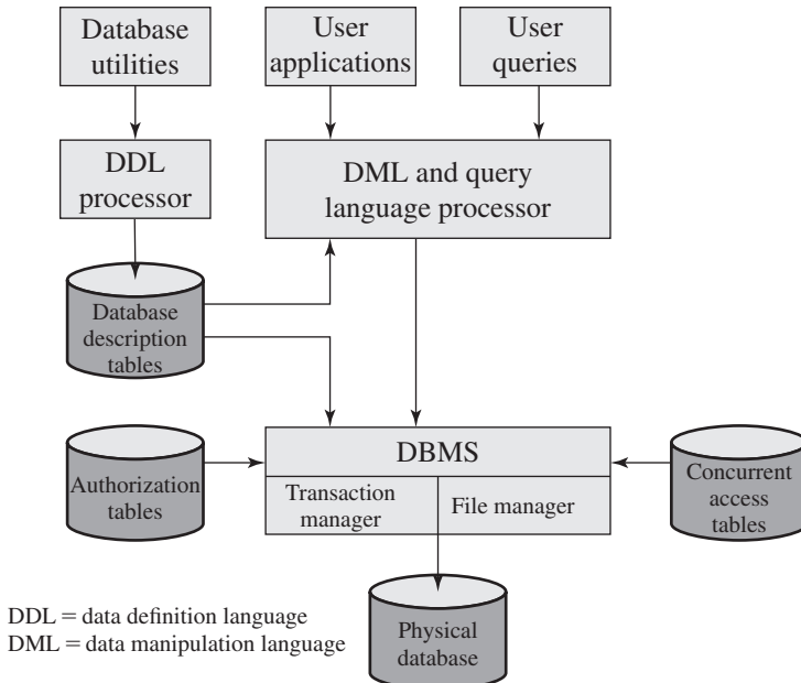
Figure 5.1 DBMS Architecture
