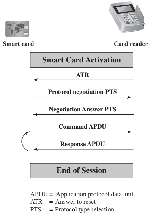
Figure 3.5 Smart Card/Reader Exchange
