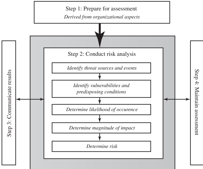
Figure 14.3 Risk Assessment Process
