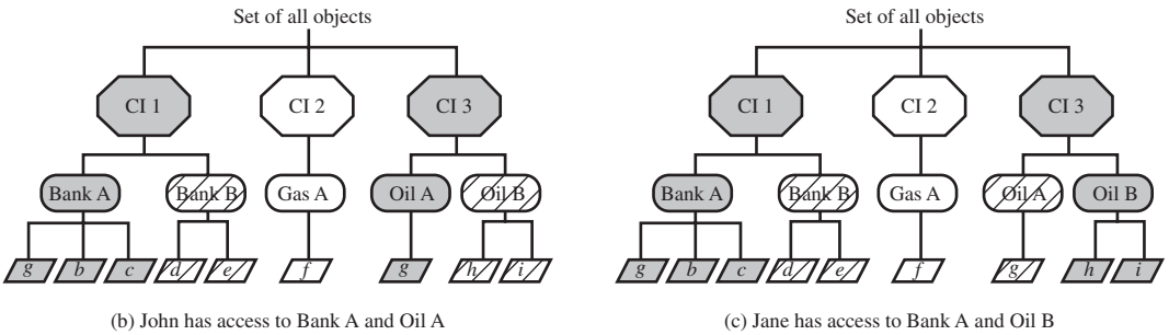
Figure 13.6 Potential Flow of Information between Two CIs
