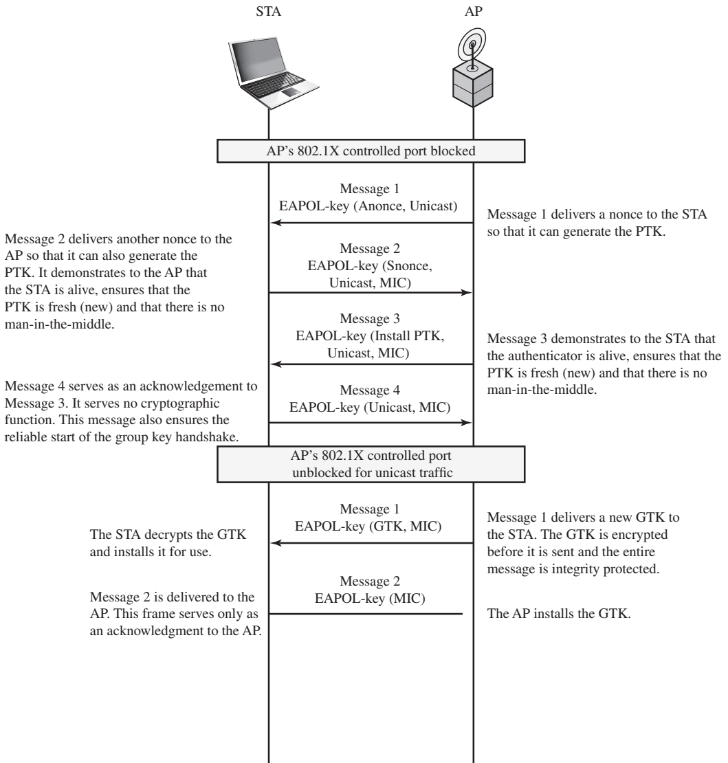
Figure 24.11 IEEE 802.11i Phases of Operation: Four-Way Handshake and Group Key Handshake
