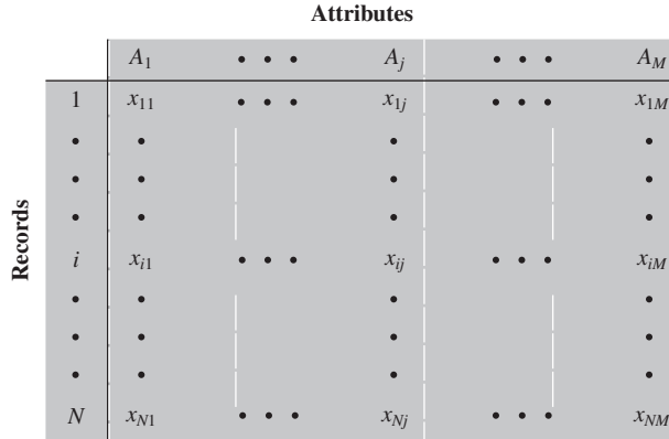
Figure 5.3 Abstract Model of a Relational Database
