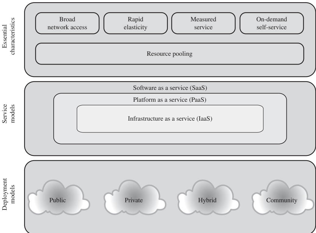
Figure 5.11 Cloud Computing Elements
