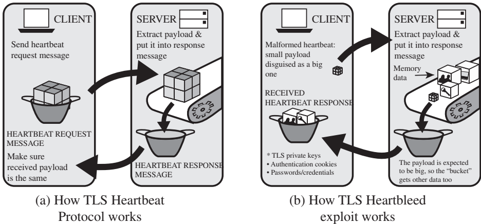
Figure 22.7 The Heartbleed Exploit
