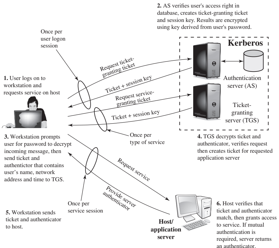
Figure 23.1 Overview of Kerberos
