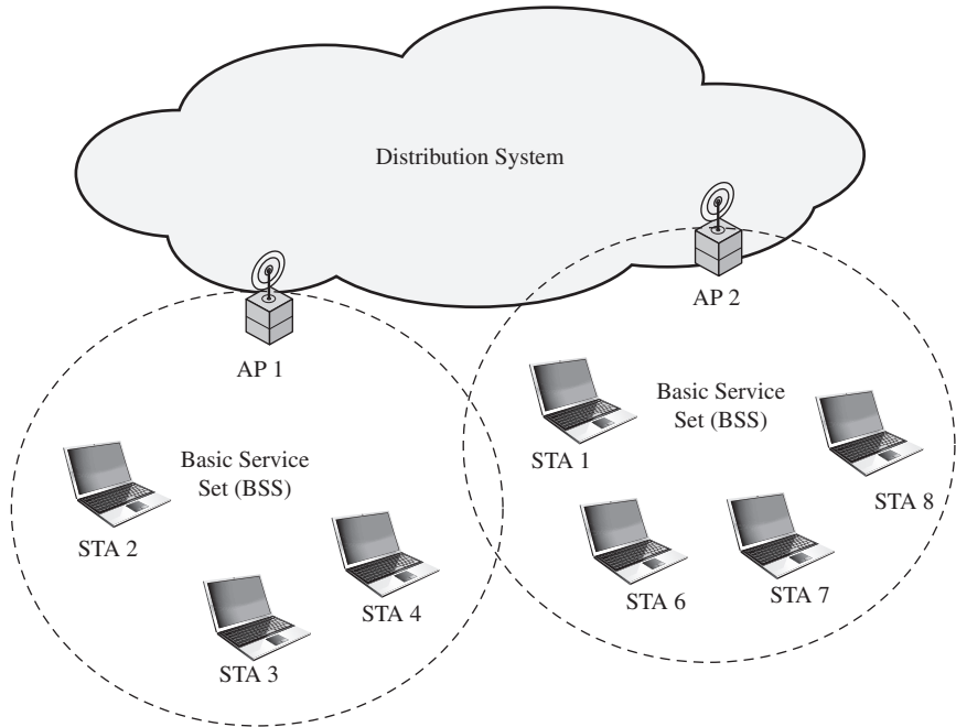
Figure 24.5 IEEE 802.11 Extended Service Set
