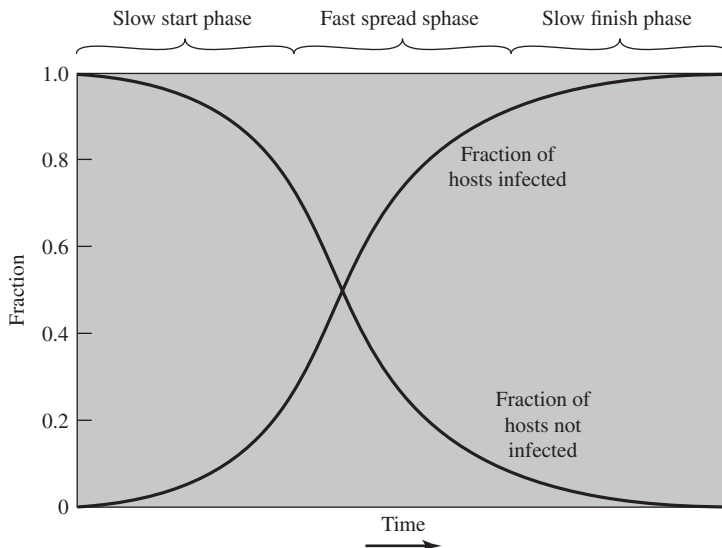
Figure 6.3 Worm Propagation Model
