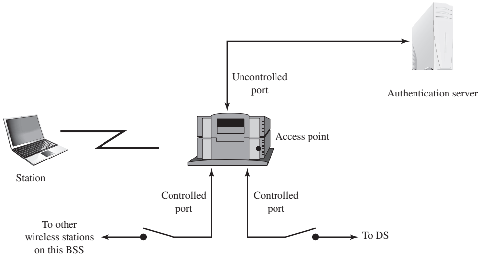
Figure 24.9 802.1X Access Control
