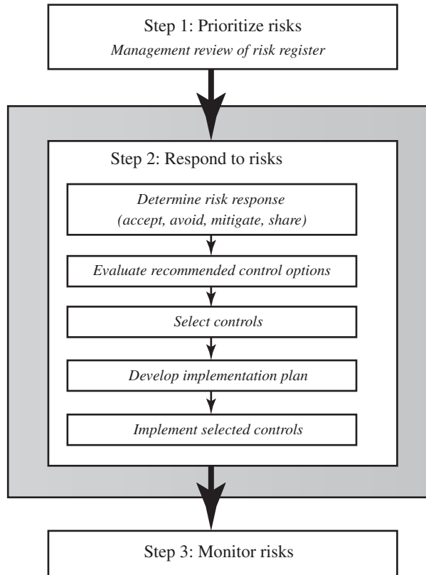
Figure 15.1 IT Security Management Controls and Implementation
