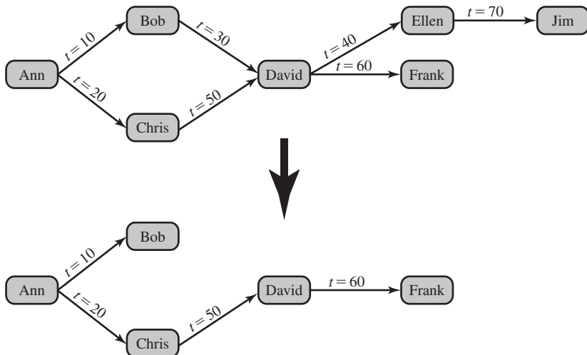
Figure 5.6 Bob Revokes Privilege from David
