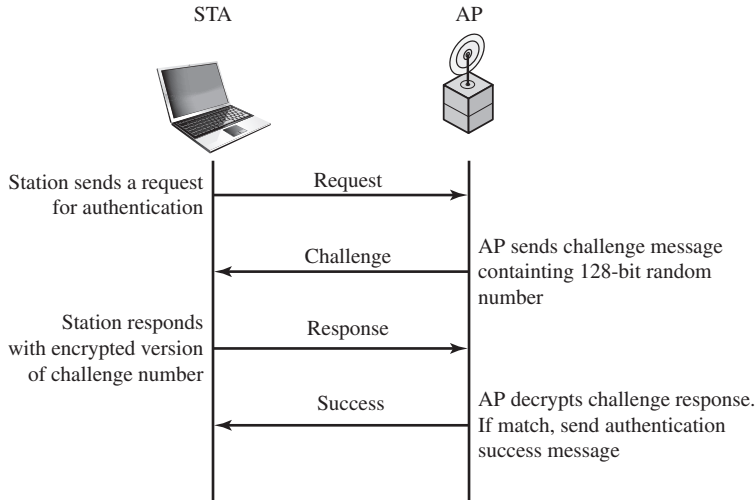
Figure 24.13 WEP Authentication
