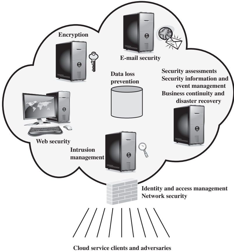
Figure 5.15 Elements of Cloud Security as a Service
