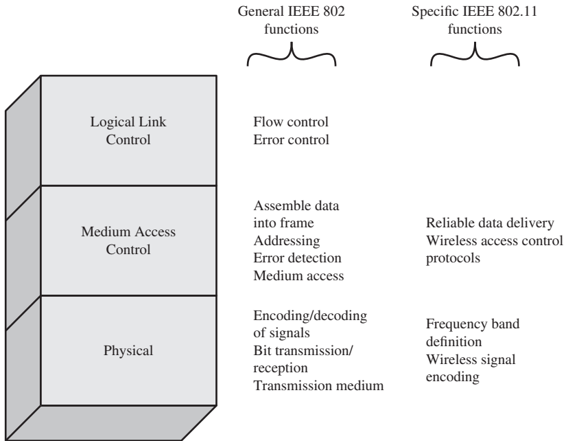
Figure 24.3 IEEE 802.11 Protocol Stack
