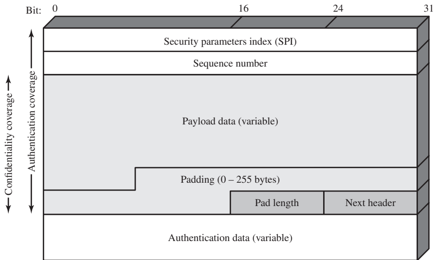
Figure 22.8 IPsec ESP Format
