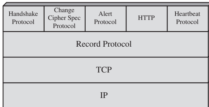
Figure 22.4 SSL/TLS Protocol Stack
