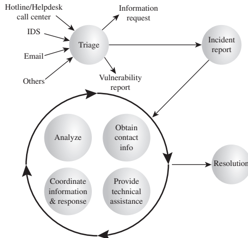
Figure 17.2 Incident Handling Life Cycle
