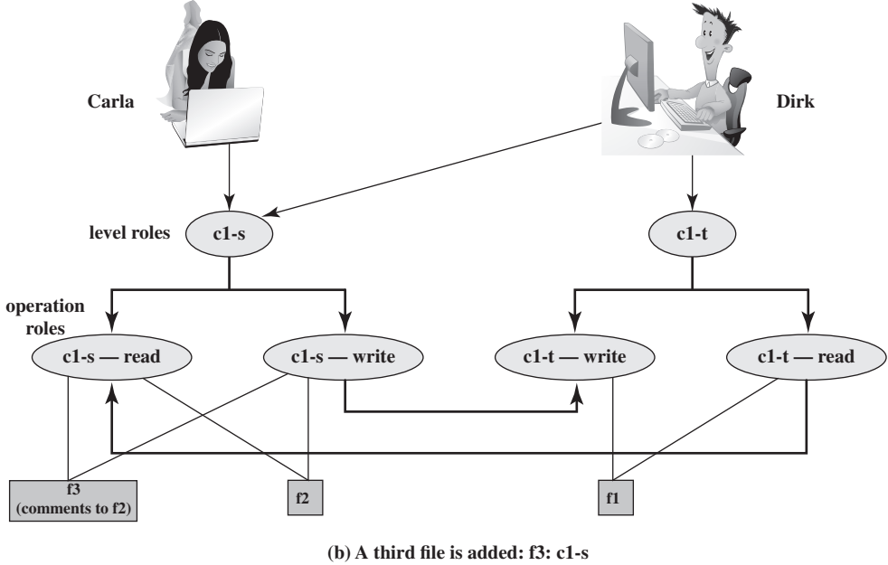
Figure 13.2 Example of Use of BLP Concepts
