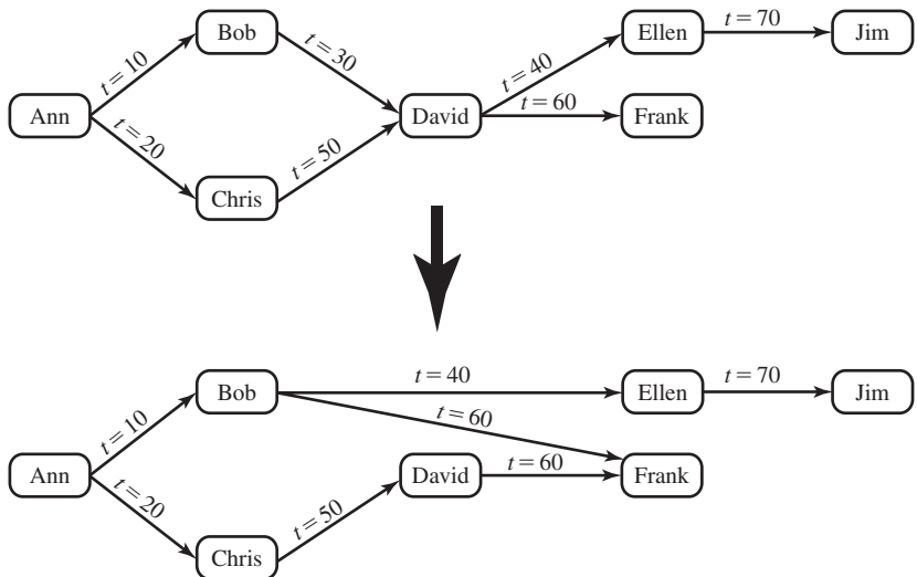
Figure 5.18 Bob Revokes Privilege from David, Second Version
