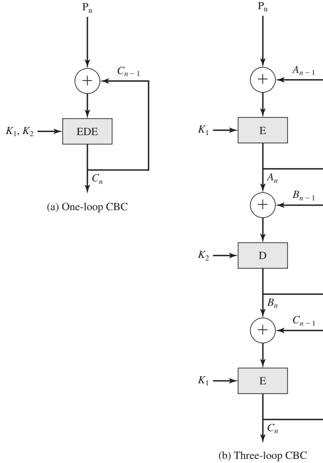
Figure 20.11 Use of Triple DES in CBC Mode
