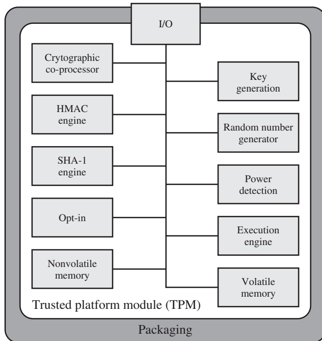
Figure 13.11 TPM Component Architecture
