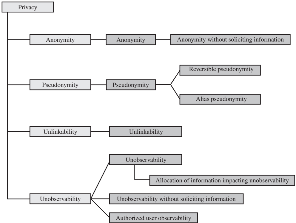
Figure 19.4 Common Criteria Privacy Class Decomposition
