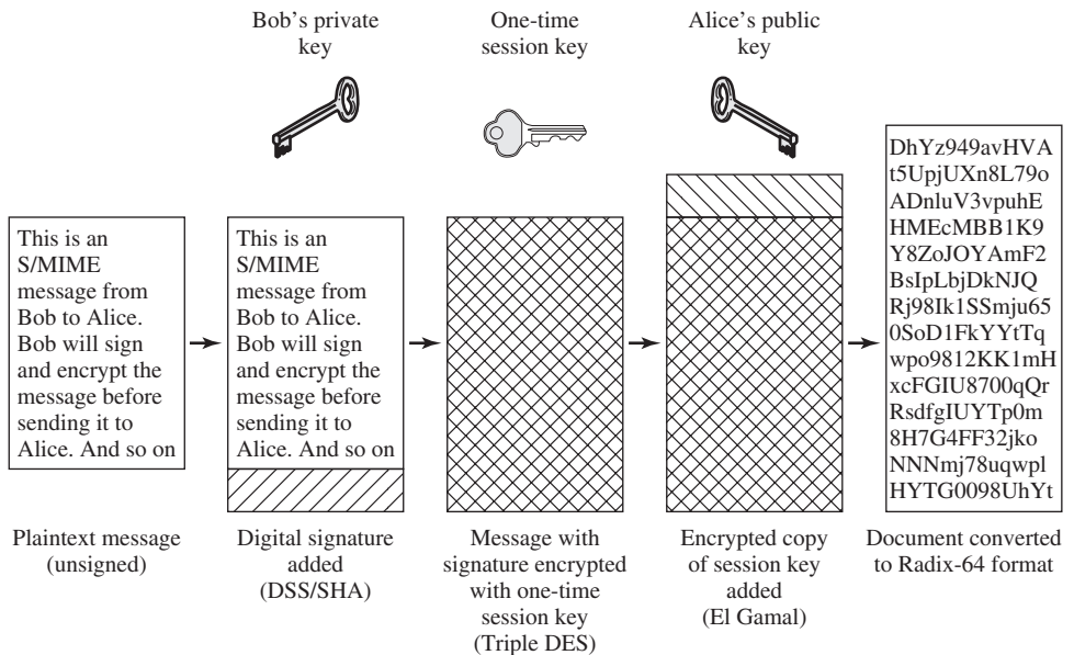
Figure 22.1 Typical S/MIME Process for Creating and S/MIME Message
