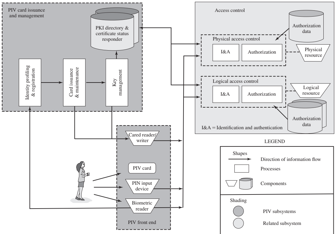
Figure 16.2 FIPS 201 PIV System Model
