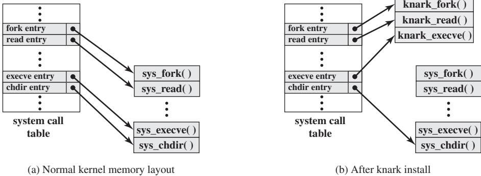
Figure 6.4 System Call Table Modification by Rootkit
