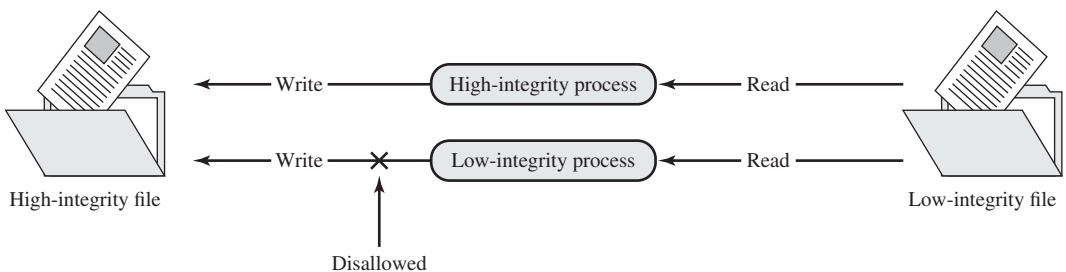
Figure 13.4 Contamination with Simple Integrity Controls Source: [GASS88].
