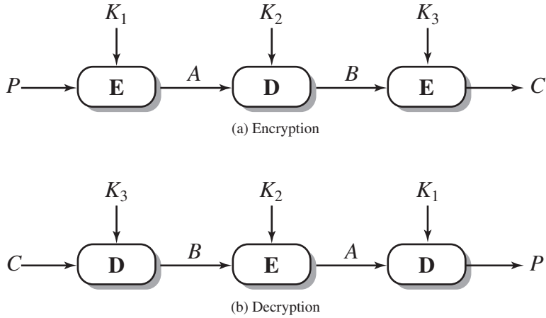
Figure 20.2 Triple DES
