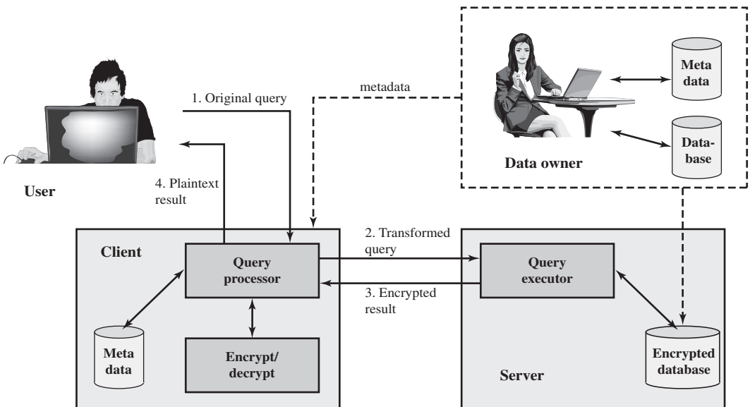
Figure 5.9 A Database Encryption Scheme
