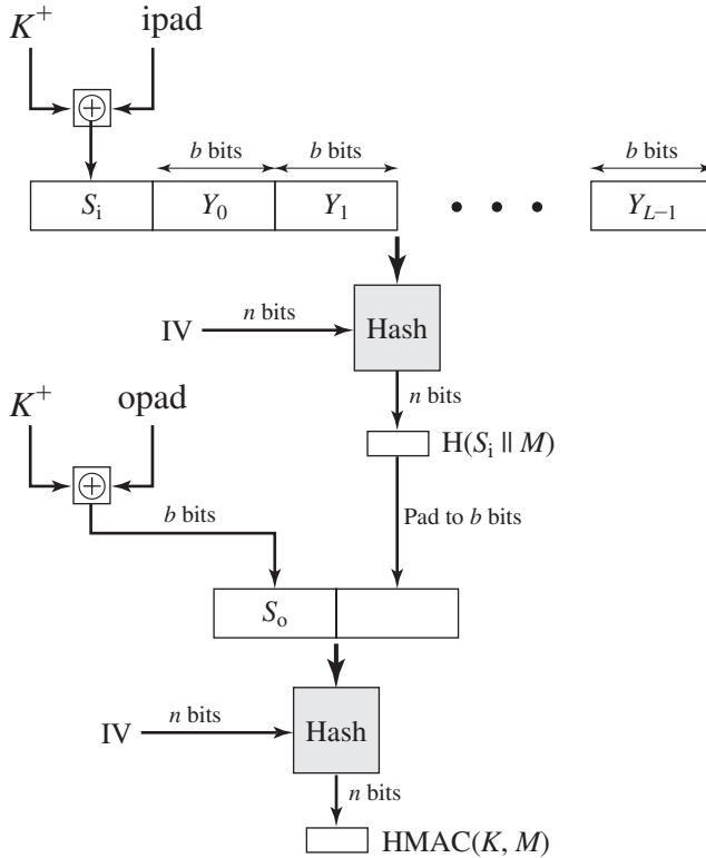
Figure 21.4 HMAC Structure
