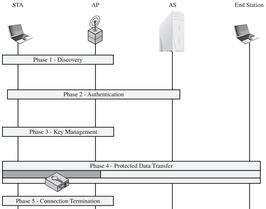
Figure 24.7 IEEE 802.11i Phases of Operation
