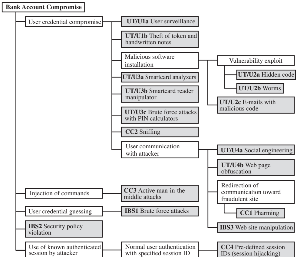
Figure 1.4 An Attack Tree for Internet Banking Authentication
