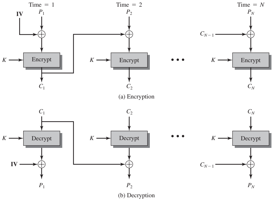
Figure 20.6 Cipher Block Chaining (CBC) Mode
