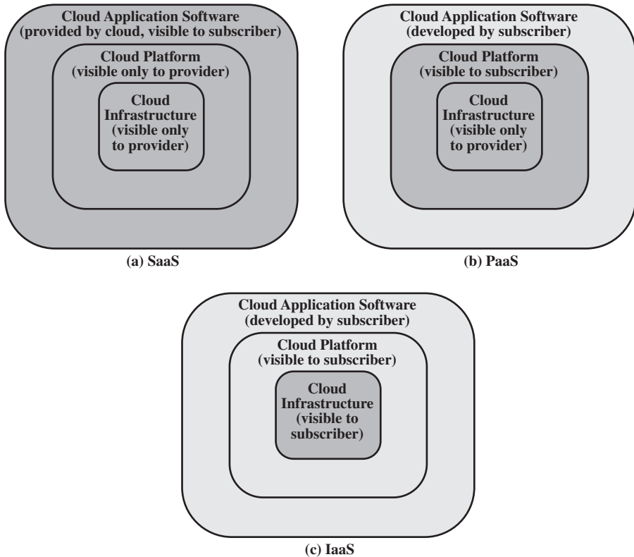
Figure 5.12 Cloud Service Models
