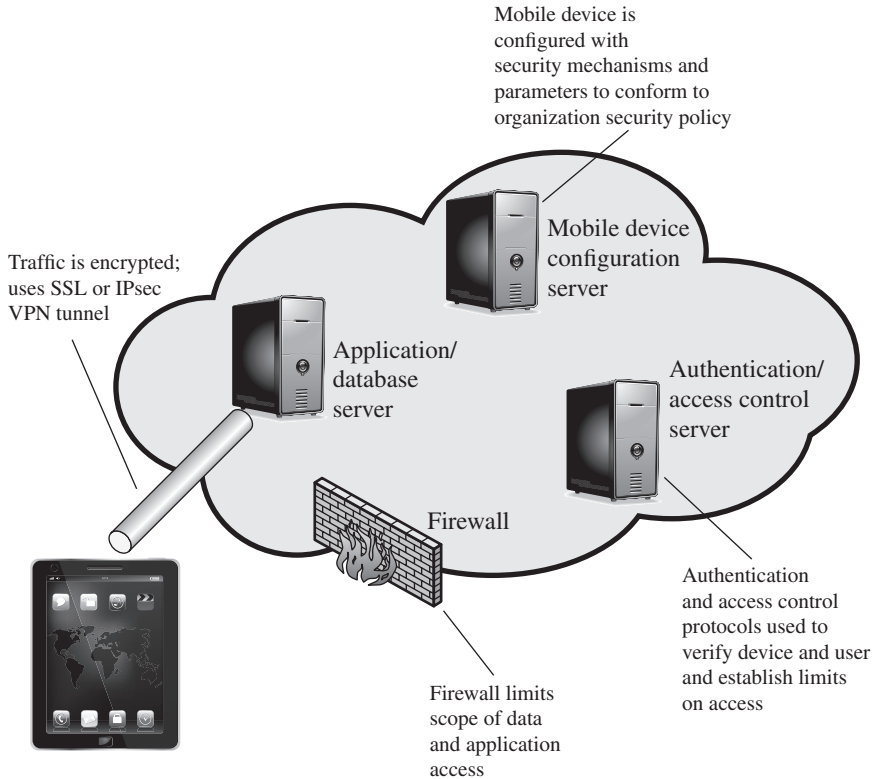
Figure 24.2 Mobile Device Security Elements
