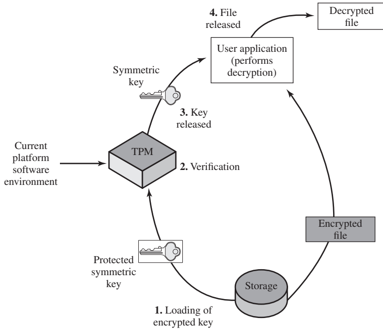
Figure 13.12 Decrypting a File Using a Protected Key
