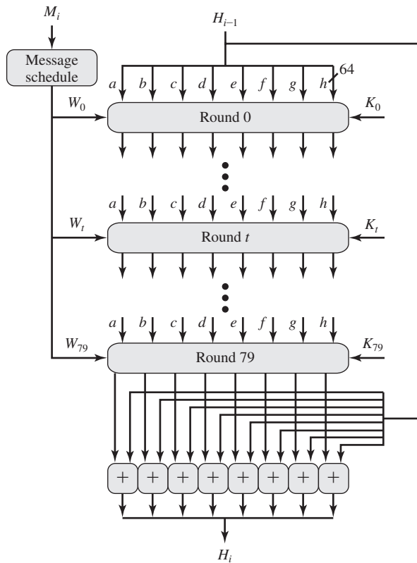
Figure 21.3 SHA-512 Processing of a Single 1024-Bit Block
