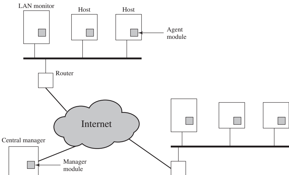
Figure 8.2 Architecture for Distributed Intrusion Detection
