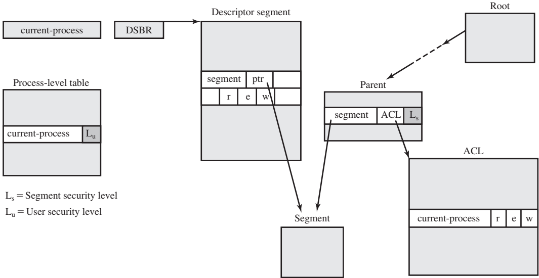
Figure 13.3 Multics Data Structures for MLS
