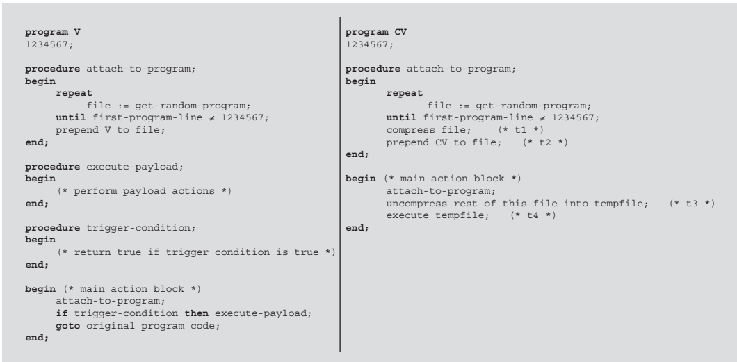
(a) A simple virus
