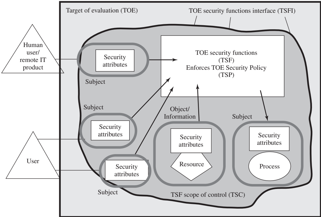
Figure 13.14 Security Functional Requirements Paradigm
