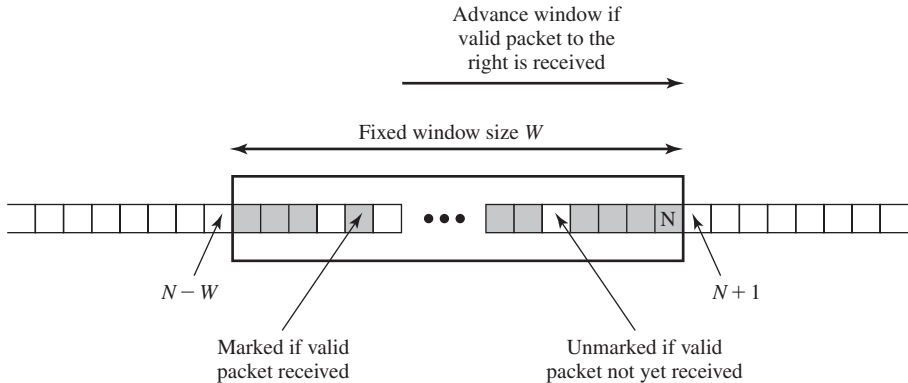
Figure 22.9 Antireplay Mechanism
