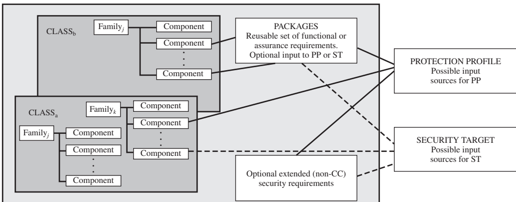
Figure 13.13 Organization and Construction of Common Criteria Requirements
