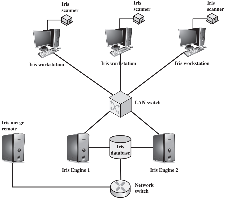
Figure 3.13 General Iris Scan Site Architecture for UAE System
