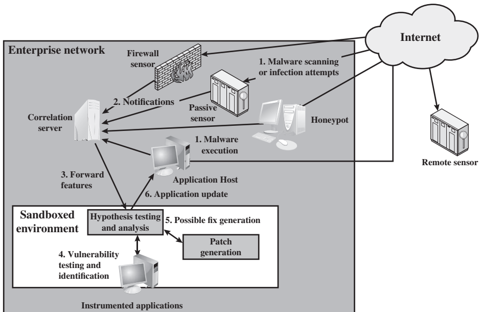
Figure 9.5 Placement of Malware Monitors (adapted from [SIDI05])
