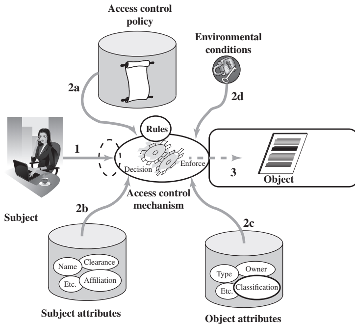
Figure 4.10 Simple ABAC Scenario
