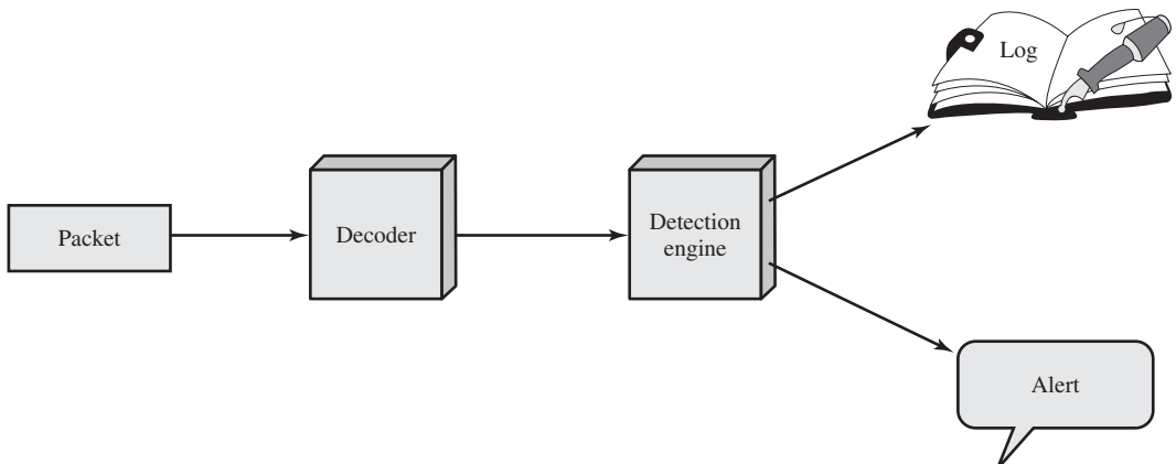
Figure 8.9 Snort Architecture
