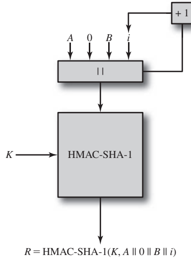
Figure 24.12 IEEE 802.11i Pseudorandom Function
