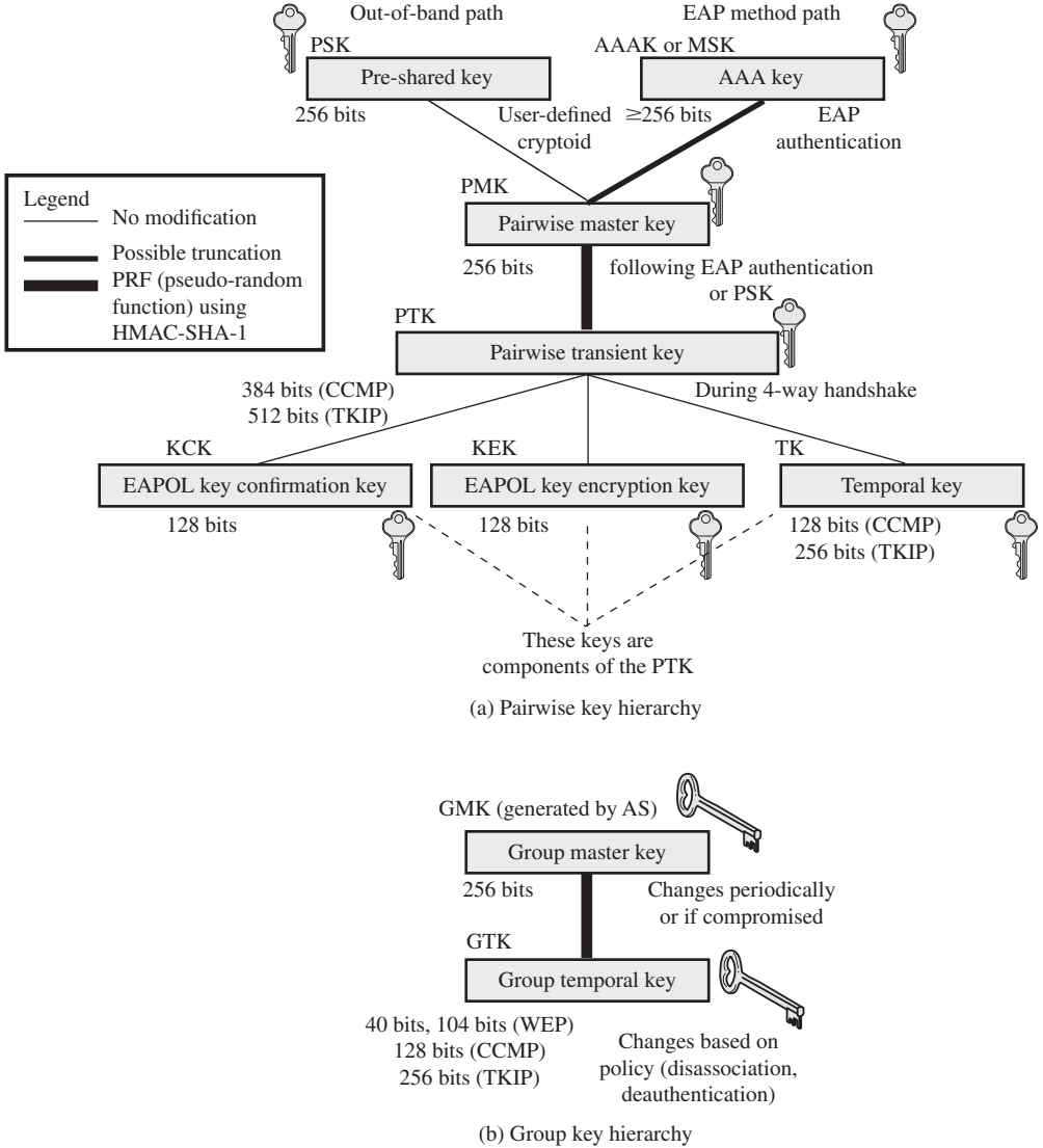
Figure 24.10 IEEE 802.11i Key Hierarchies
