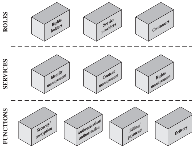
Figure 19.3 DRM System Architecture
